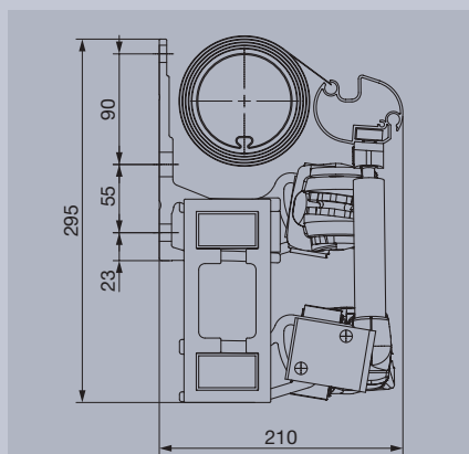
Montage mural Topas® MiniMax
